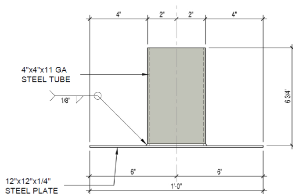
Figure 2: Steel Tube and Baseplate Assembly
